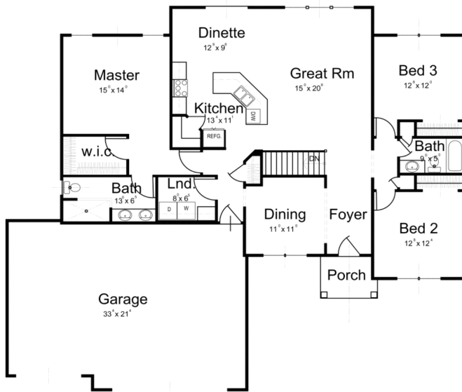
First Floor Plan 1,834 sq.ft. Living Area
